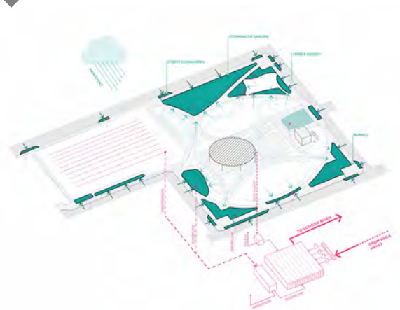
Figure 62. Stormwater management system design diagram for Northwest Resilience Park in Hoboken, NJ
