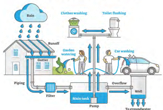
Figure 46. Diagram on the mechanics of rainwater harvesting; Adobe Stock
